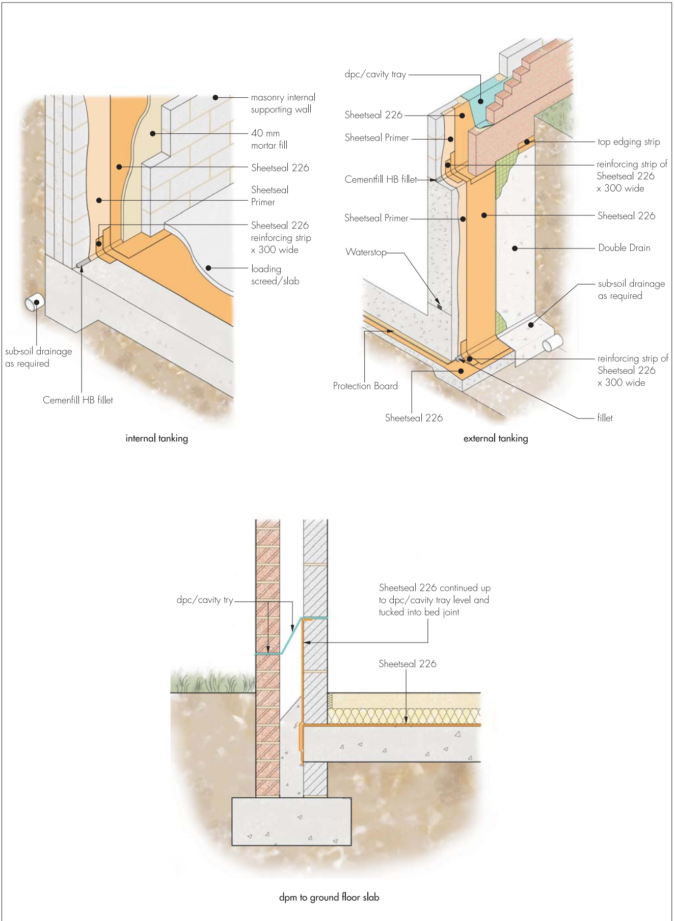
Figure 1 Installation details
