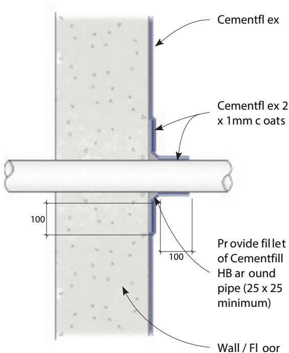
Pipe Entry Detail
