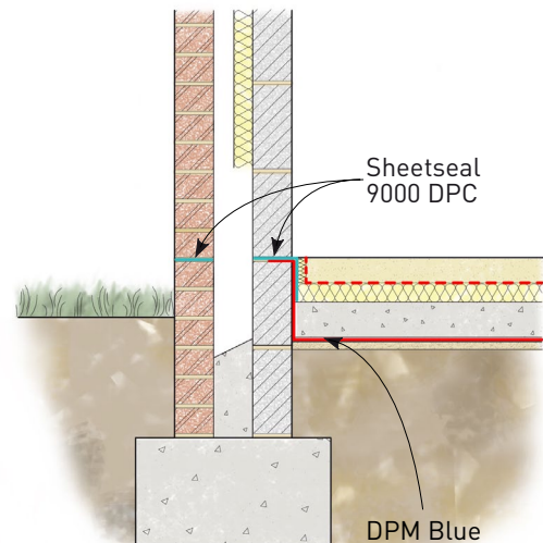
Typical Ground Bearing Slab
