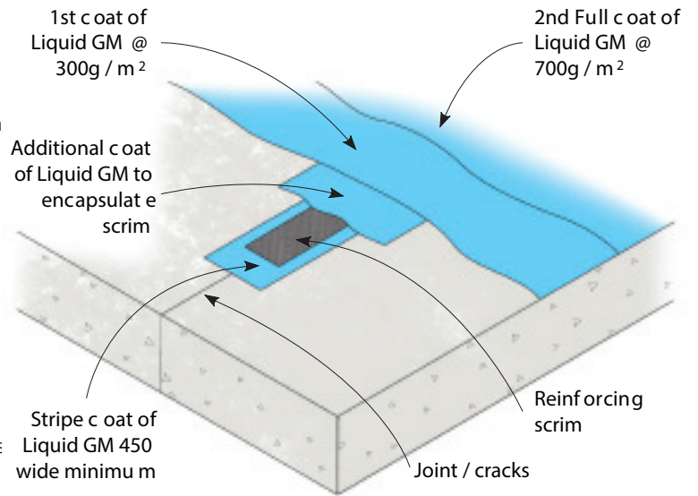
Typical Joint Detail
