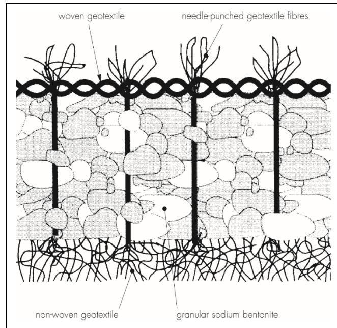
Figure 1 Cross-section through RIW Structureseal
