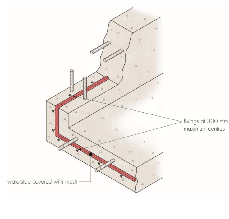
Figure 2 RIW Waterstop installation details
